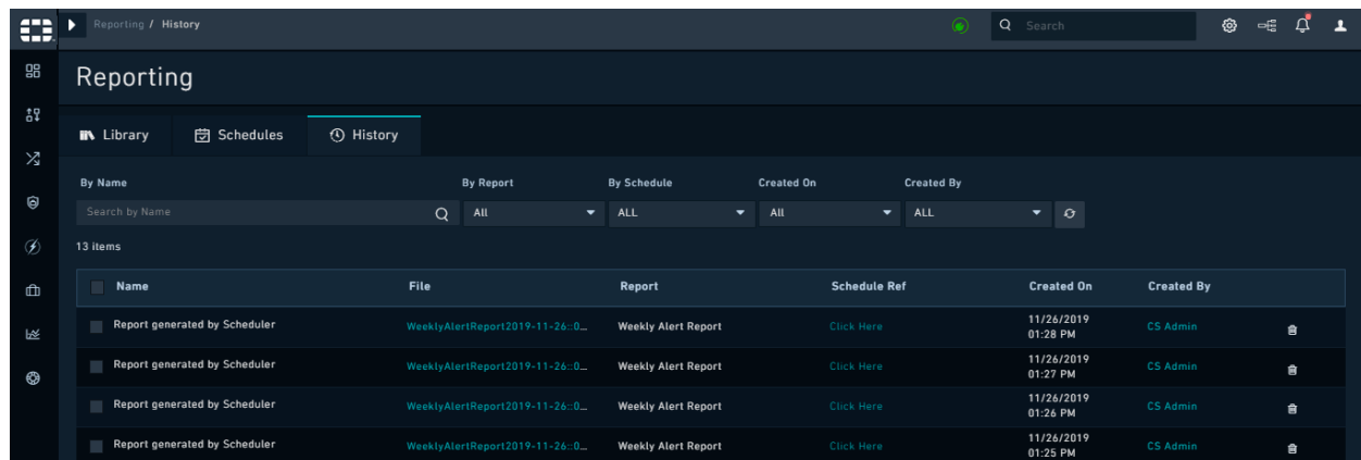
Figure 193. Historical Reports
