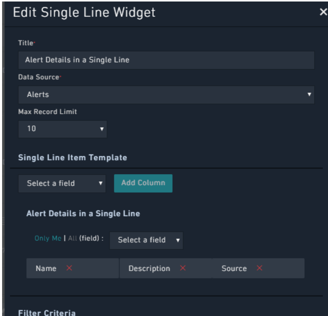
Figure 85. List Widget
