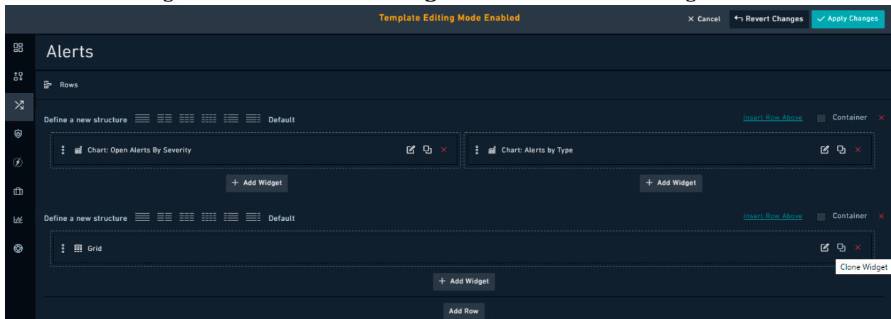
Figure 41. Editing Widgets
