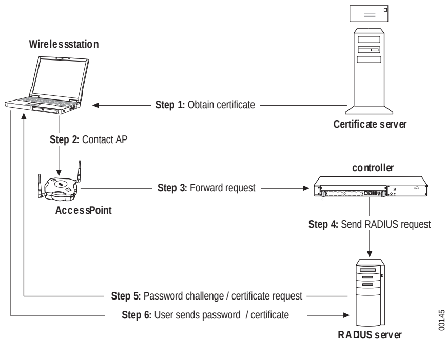
Figure 53: Conceptual Model for 802.1X RADIUS Server Authentication
