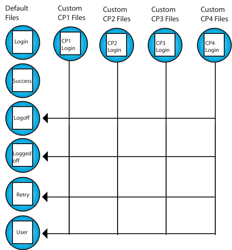
Figure 59: Captive Portal HTML Pages (maximum)
